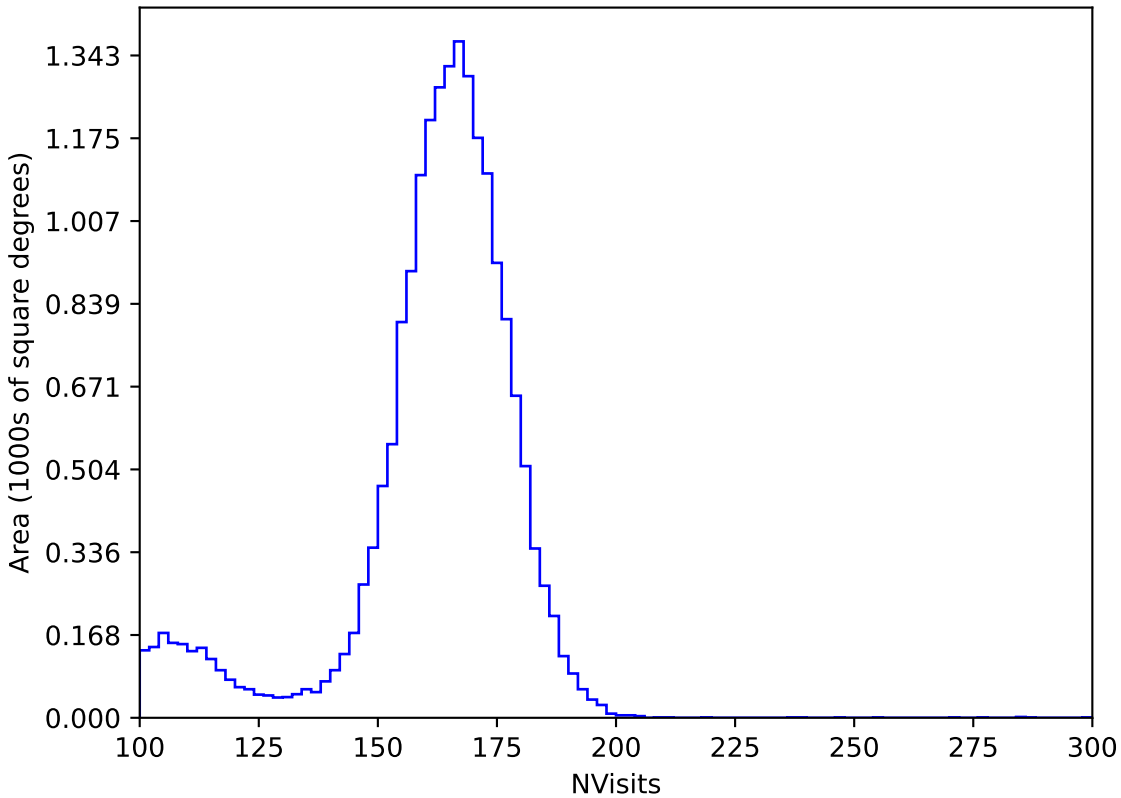
baseline_v3.0_10yrs All sky y band: NVisits
