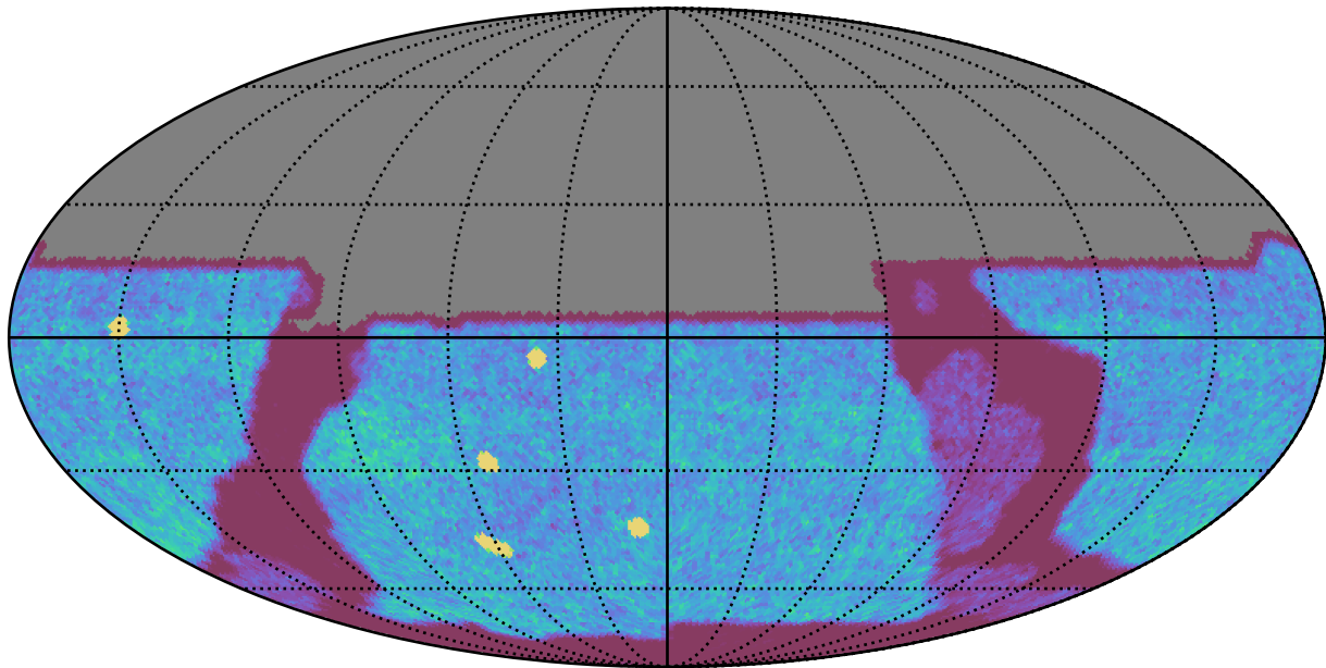
baseline_v3.0_10yrs All sky u band: NVisits
