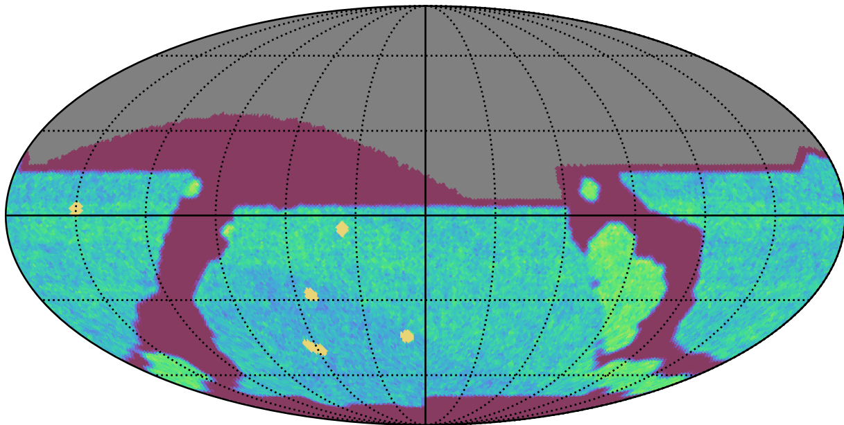
baseline_v3.0_10yrs All sky r band: NVisits
