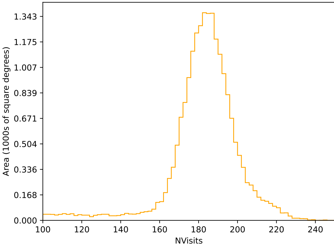
baseline_v3.0_10yrs All sky r band: NVisits
