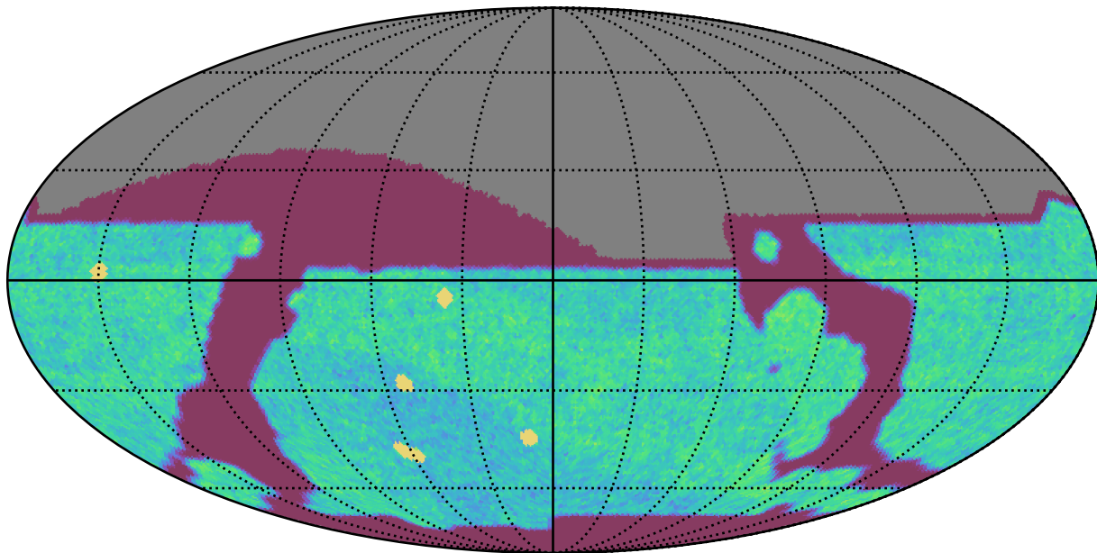
baseline_v3.0_10yrs All sky i band: NVisits
