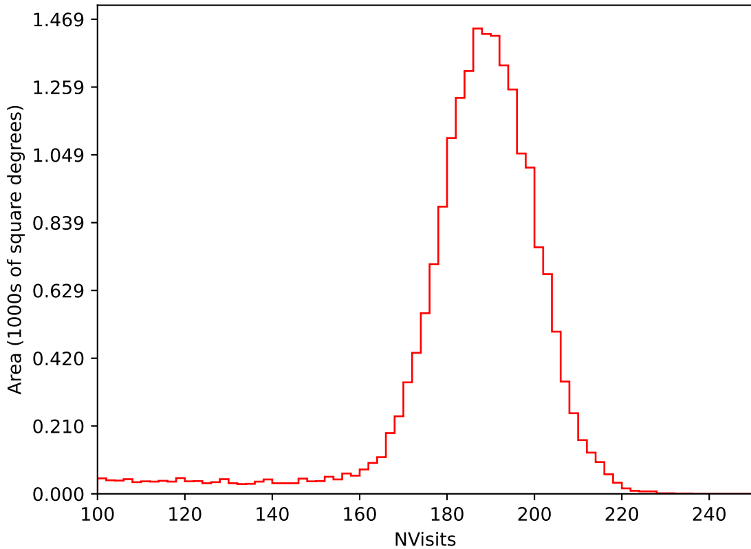
baseline_v3.0_10yrs All sky i band: NVisits
