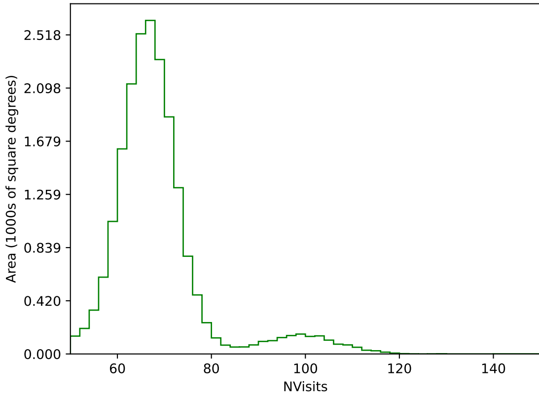
baseline_v3.0_10yrs All sky g band: NVisits
