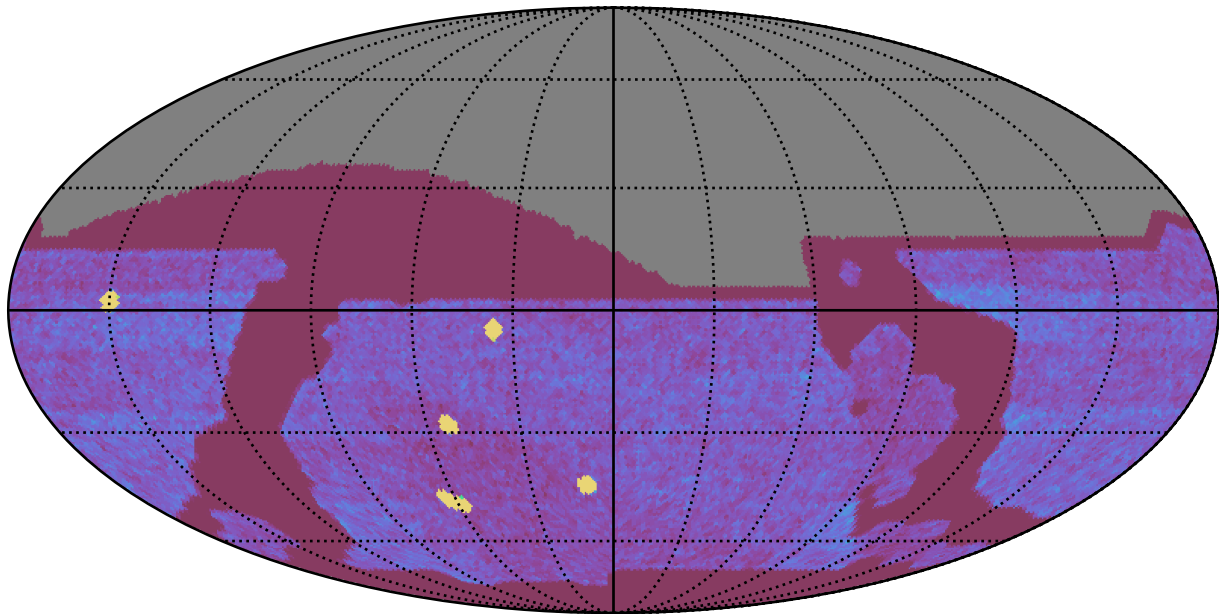
baseline_v3.0_10yrs All sky all bands: NVisits
