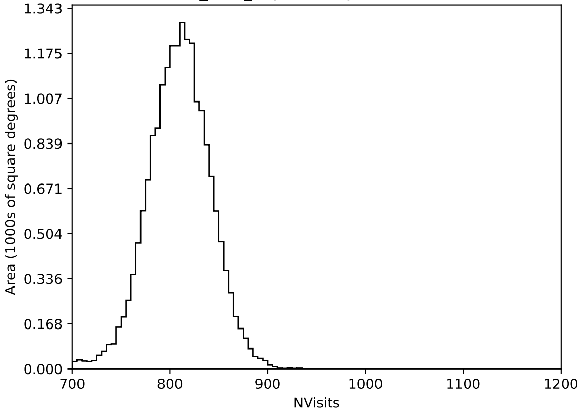
baseline_v3.0_10yrs All sky all bands: NVisits
