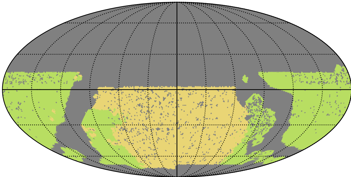
baseline_v3.0_10yrs WFD all bands: NSeasons
