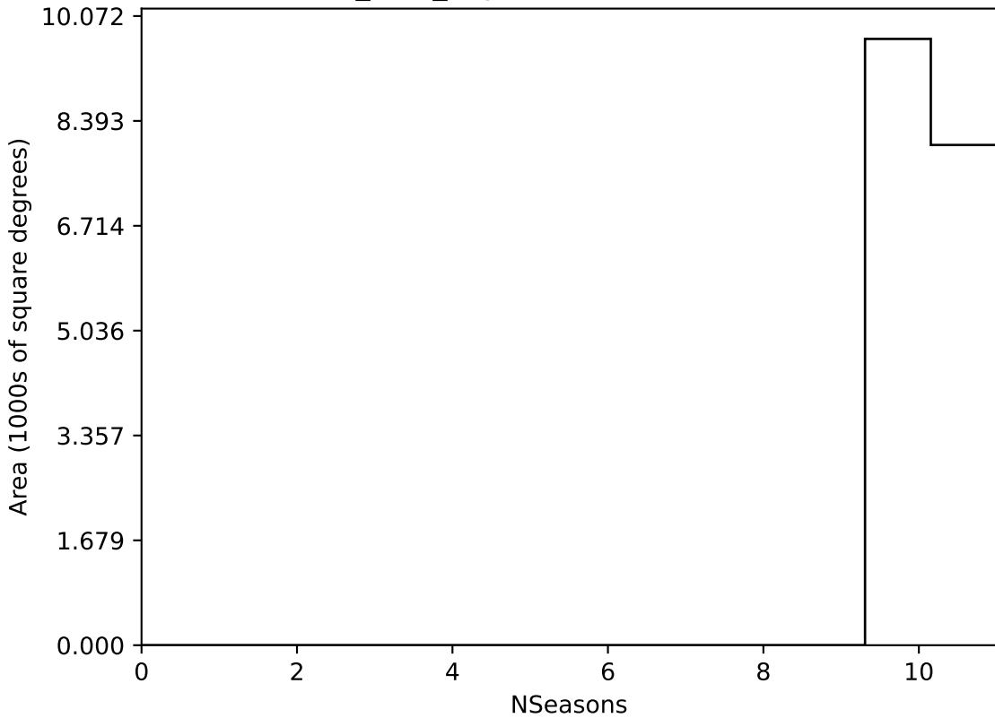
baseline_v3.0_10yrs WFD all bands: NSeasons
