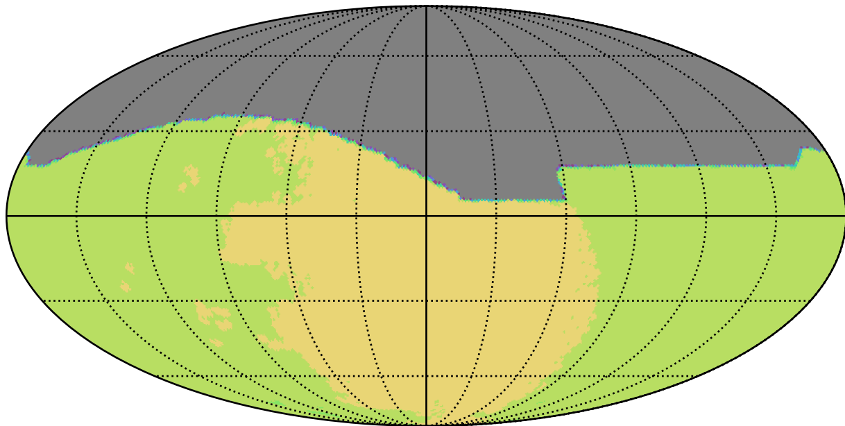
baseline_v3.0_10yrs All sky all bands: NSeasons
