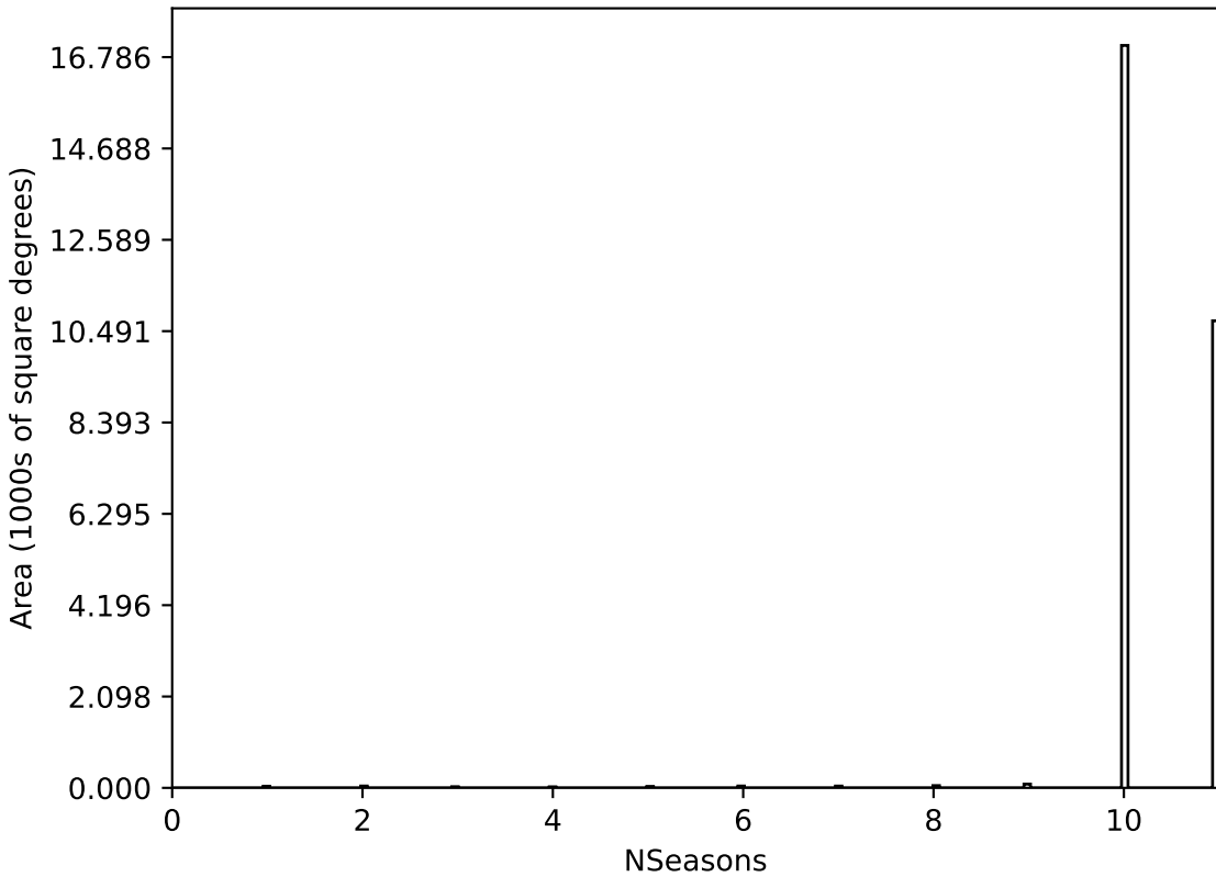
baseline_v3.0_10yrs All sky all bands: NSeasons
