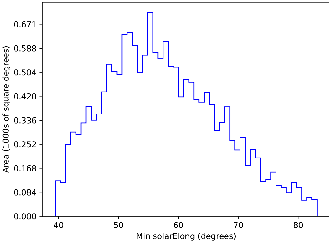
baseline_v3.0_10yrs WFD z band: Min solarElong
