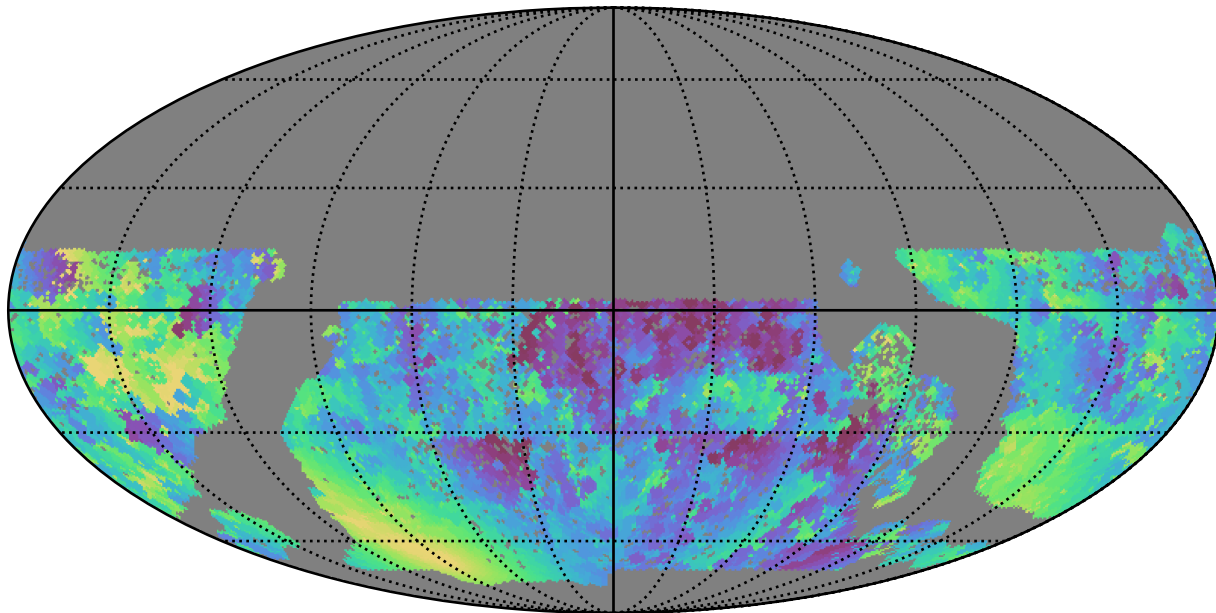
baseline_v3.0_10yrs WFD y band: Min solarElong
