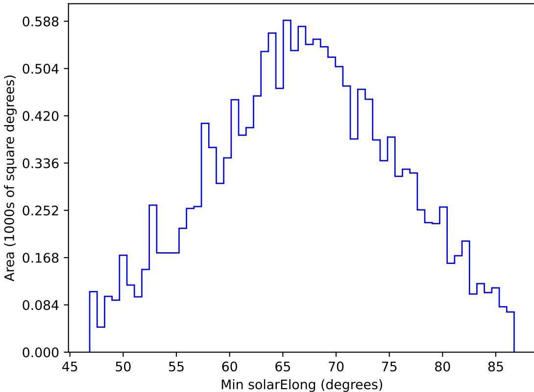
baseline_v3.0_10yrs WFD y band: Min solarElong
