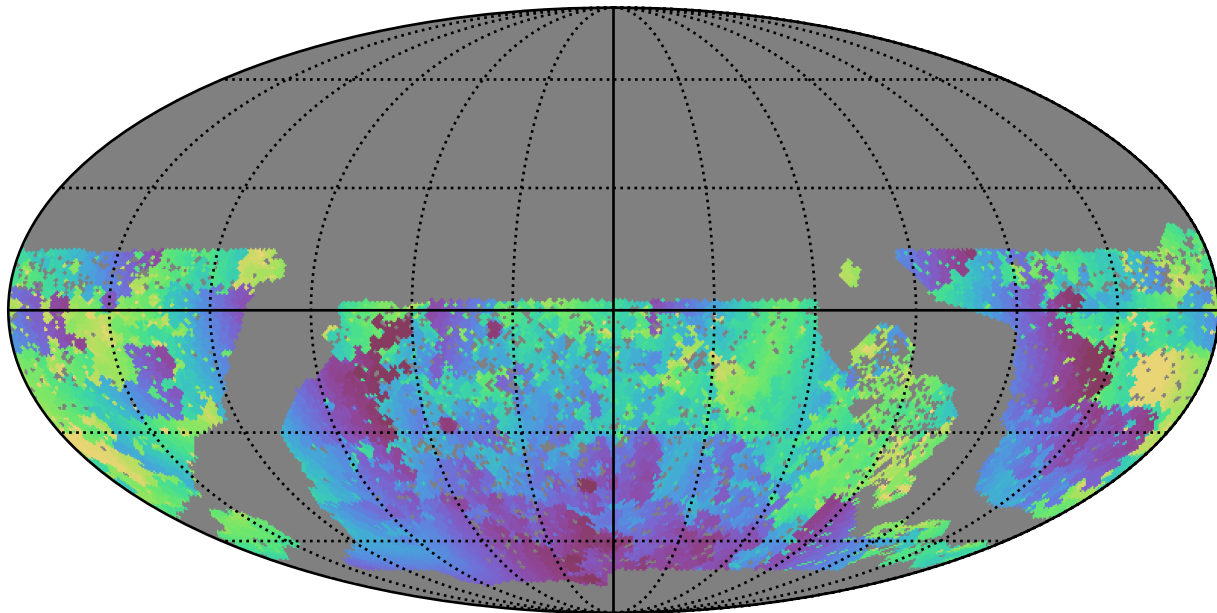
baseline_v3.0_10yrs WFD u band: Min solarElong
