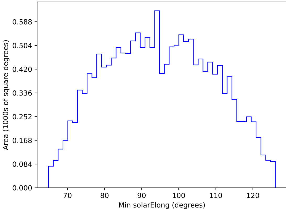
baseline_v3.0_10yrs WFD u band: Min solarElong
