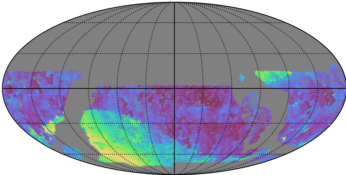
baseline_v3.0_10yrs WFD r band: Min solarElong
