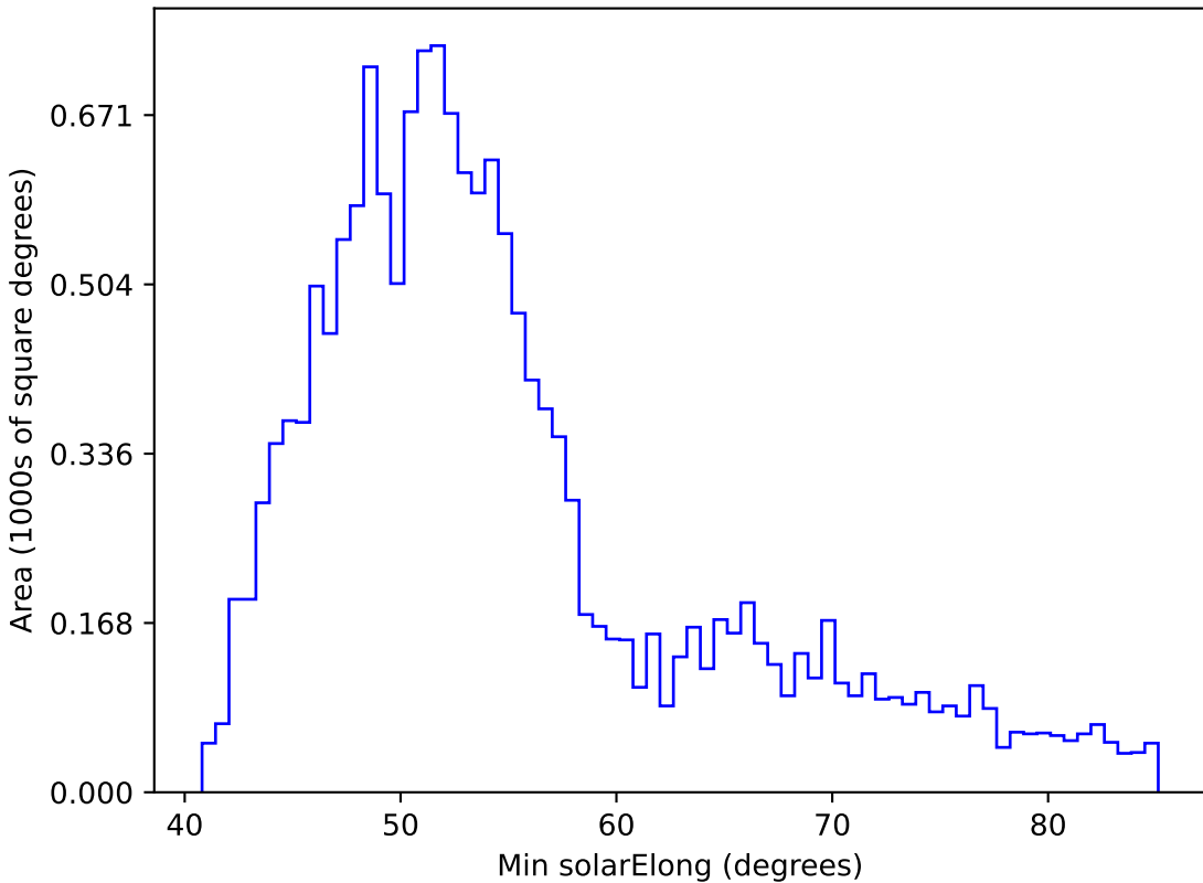
baseline_v3.0_10yrs WFD r band: Min solarElong
