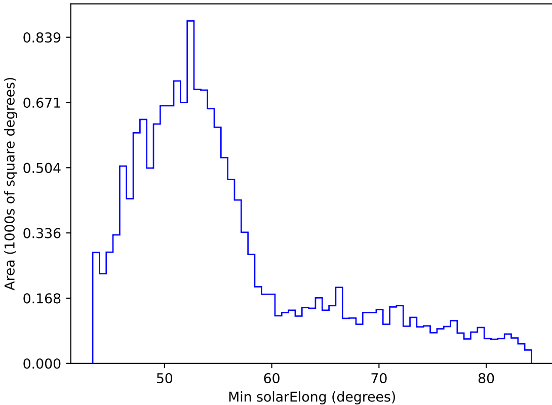
baseline_v3.0_10yrs WFD i band: Min solarElong
