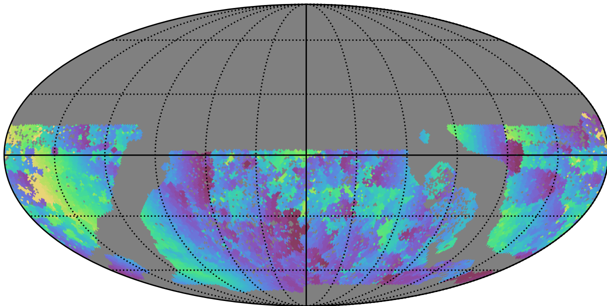
baseline_v3.0_10yrs WFD g band: Min solarElong
