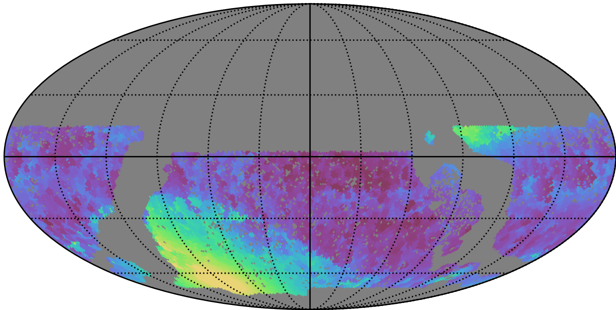
baseline_v3.0_10yrs WFD all bands: Min solarElong
