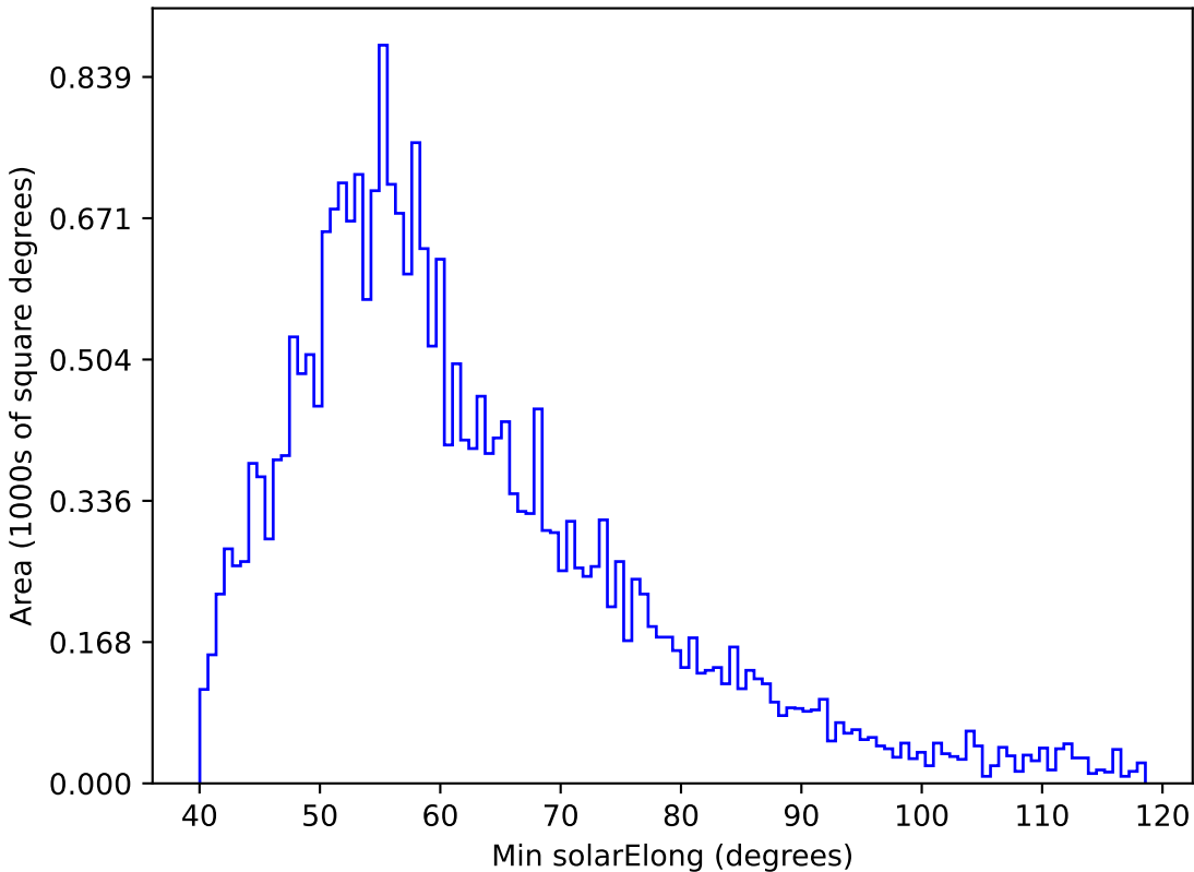
baseline_v3.0_10yrs All sky z band: Min solarElong
