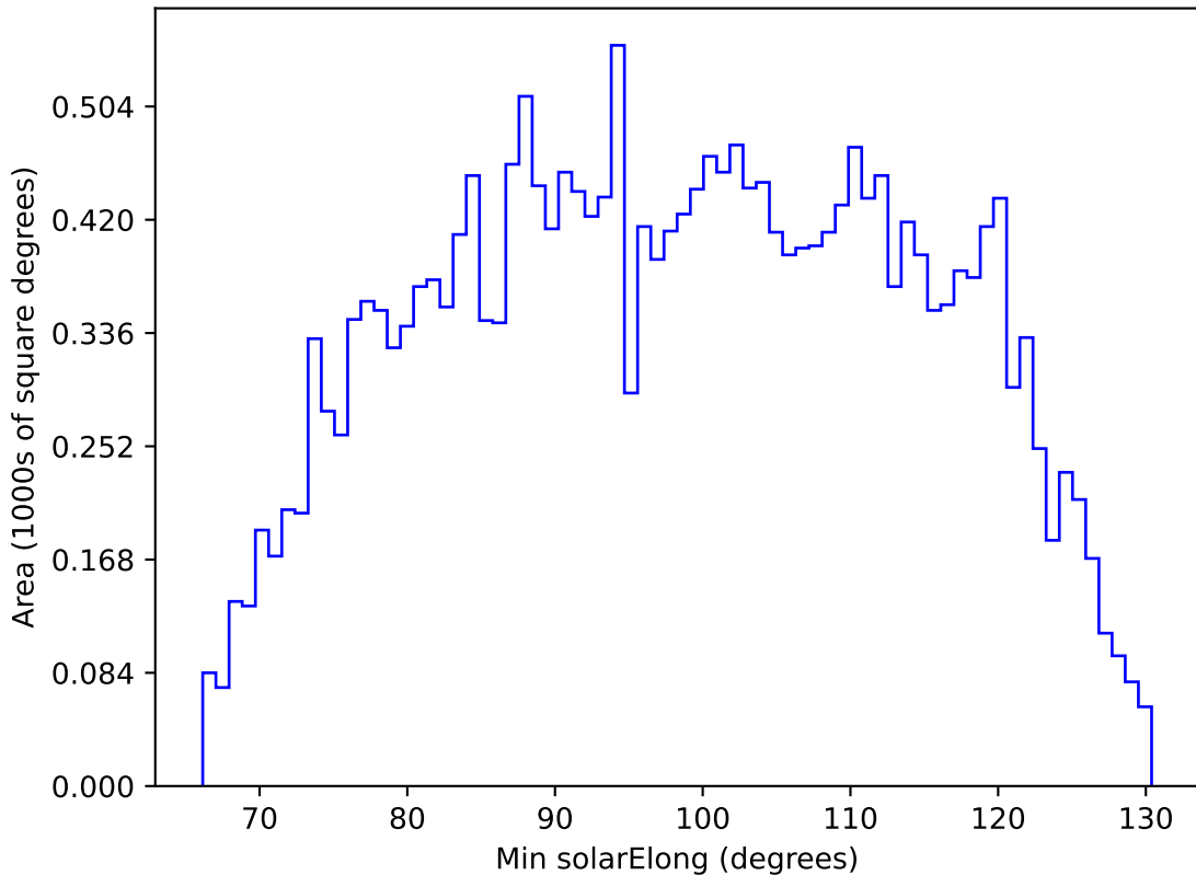
baseline_v3.0_10yrs All sky u band: Min solarElong
