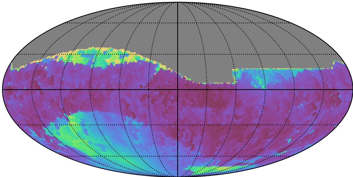
baseline_v3.0_10yrs All sky r band: Min solarElong
