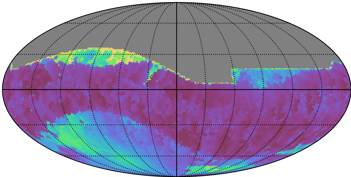
baseline_v3.0_10yrs All sky i band: Min solarElong
