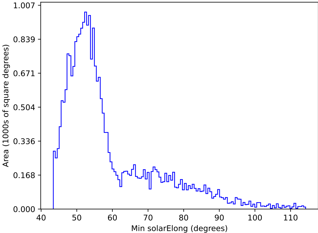
baseline_v3.0_10yrs All sky i band: Min solarElong
