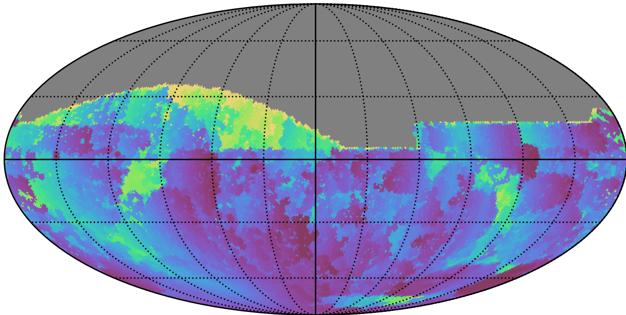
baseline_v3.0_10yrs All sky g band: Min solarElong
