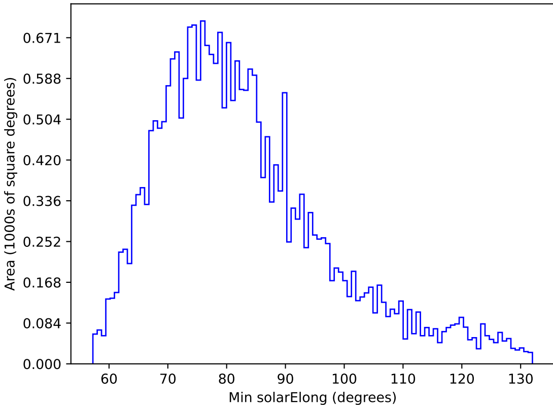
baseline_v3.0_10yrs All sky g band: Min solarElong
