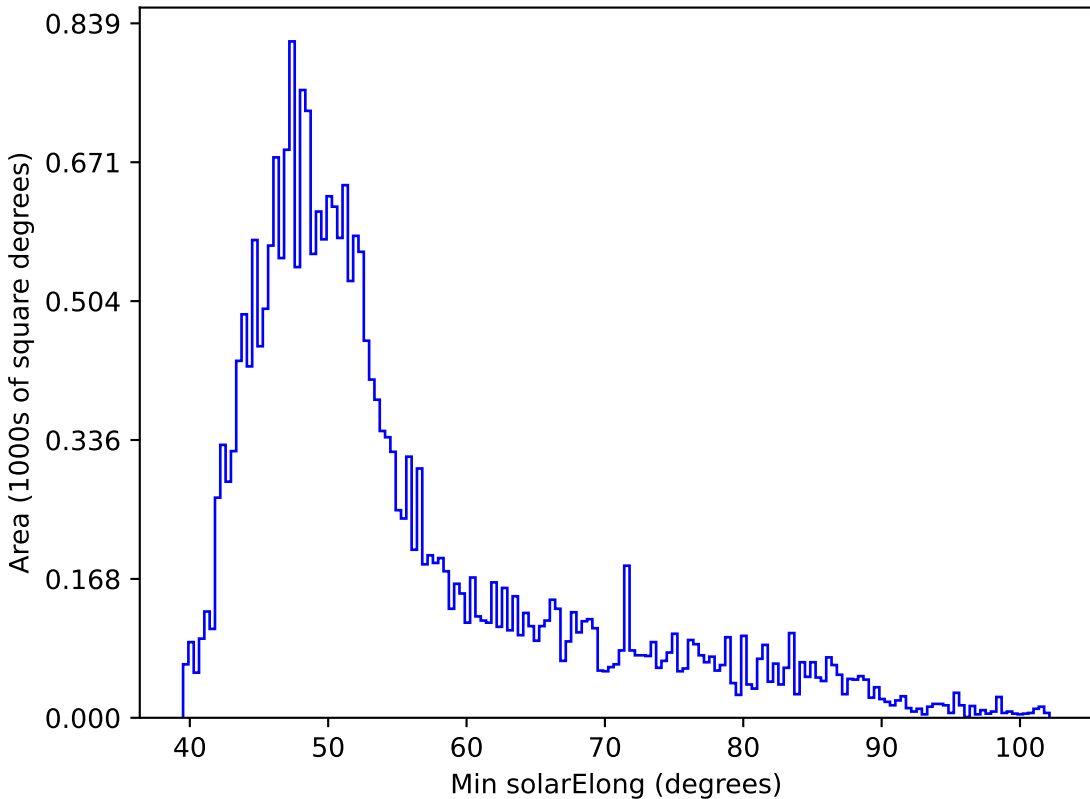
baseline_v3.0_10yrs All sky all bands: Min solarElong
