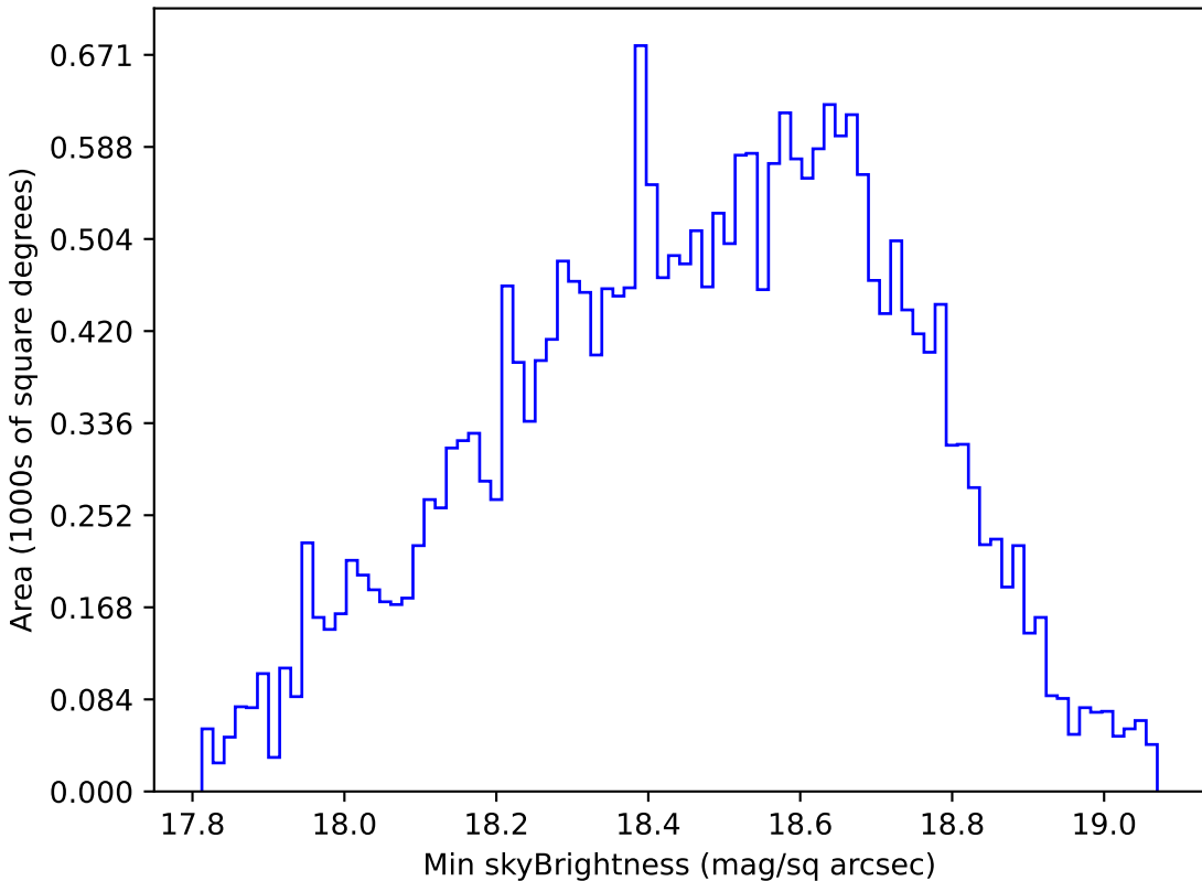
baseline_v3.0_10yrs Yr 1 z band: Min skyBrightness
