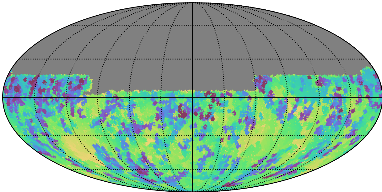
baseline_v3.0_10yrs Yr 1 y band: Min skyBrightness
