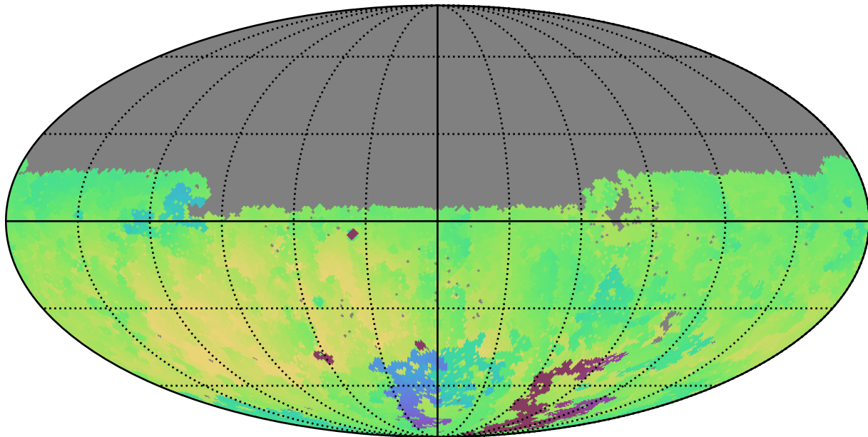
baseline_v3.0_10yrs Yr 1 u band: Min skyBrightness
