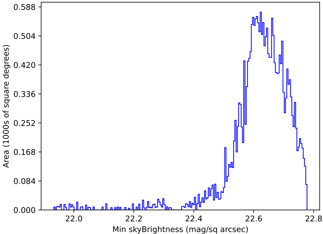
baseline_v3.0_10yrs Yr 1 u band: Min skyBrightness
