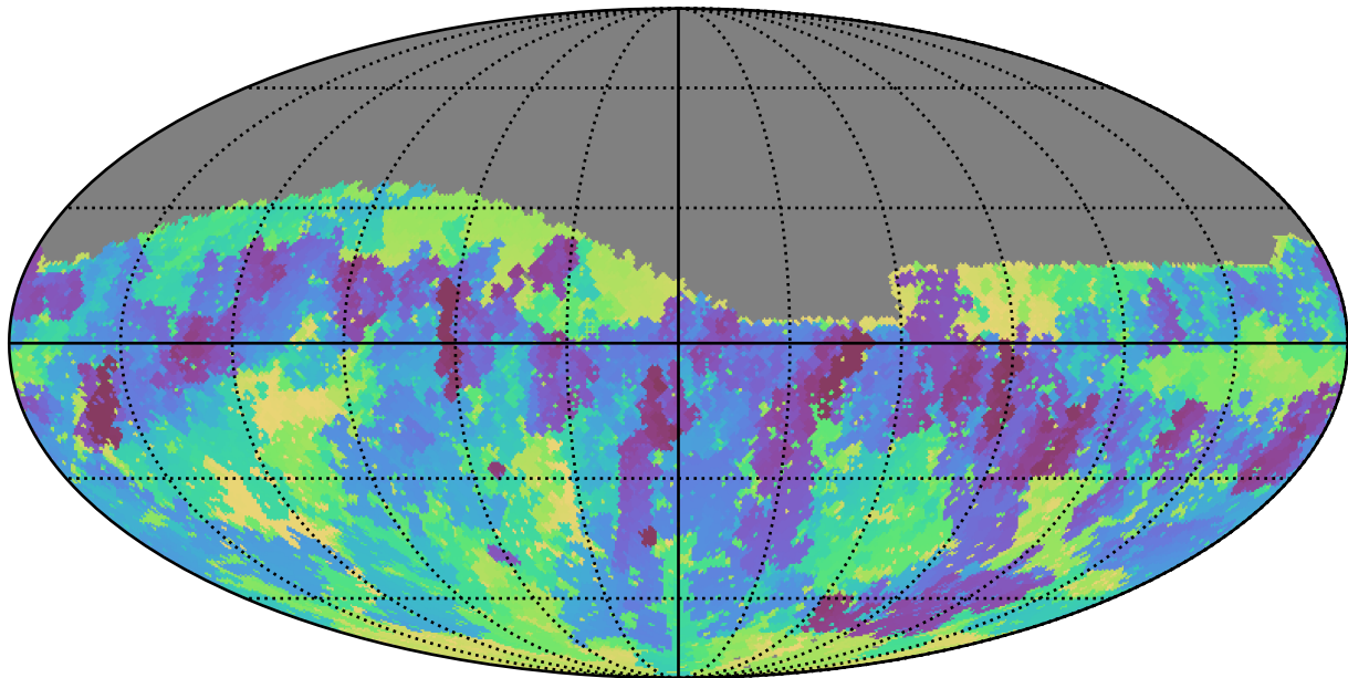
baseline_v3.0_10yrs Yr 1 r band: Min skyBrightness
