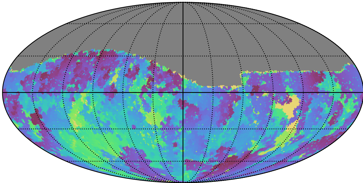
baseline_v3.0_10yrs Yr 1 i band: Min skyBrightness
