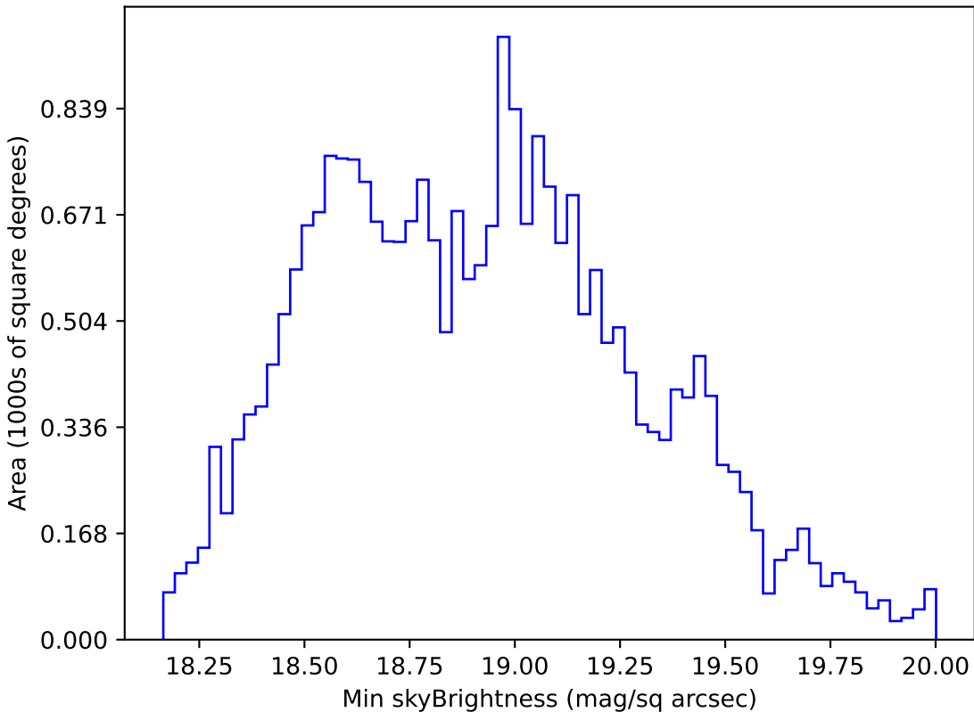
baseline_v3.0_10yrs Yr 1 i band: Min skyBrightness
