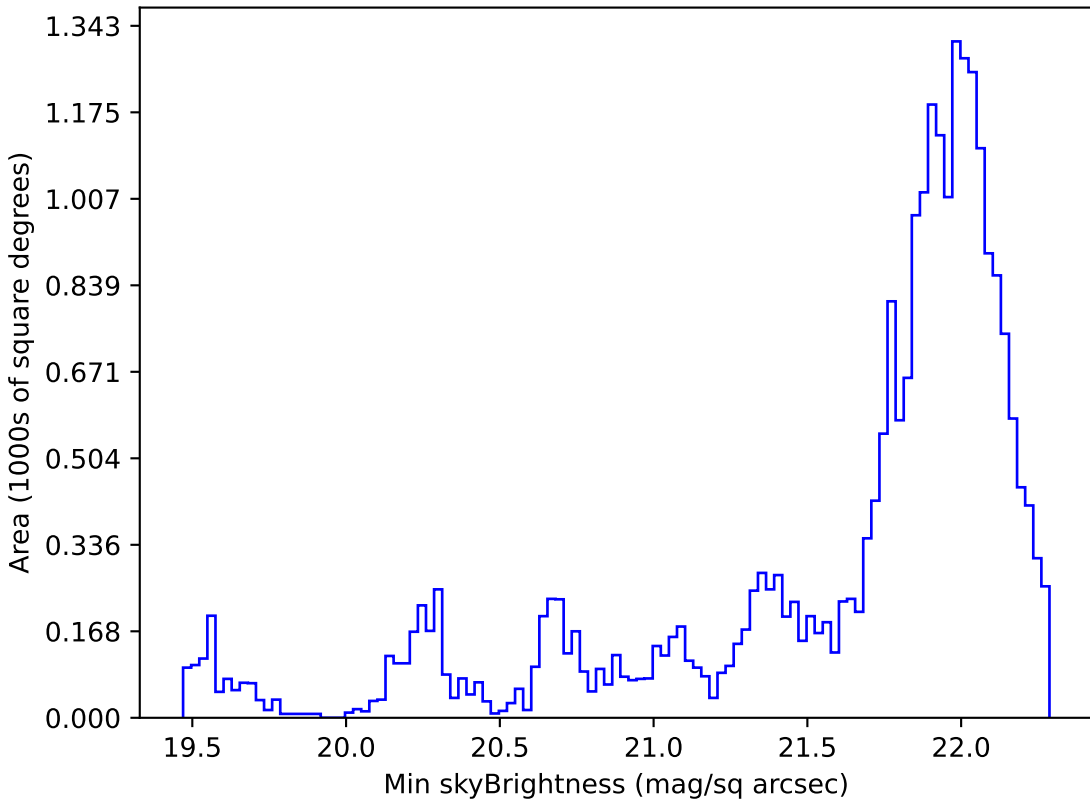
baseline_v3.0_10yrs Yr 1 g band: Min skyBrightness
