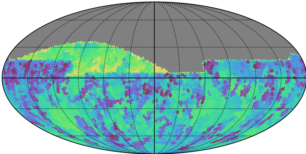
baseline_v3.0_10yrs Yr 1 all bands: Min skyBrightness
