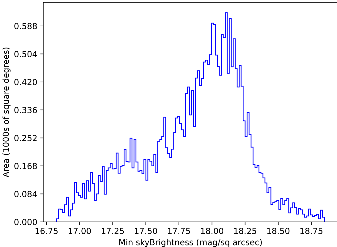
baseline_v3.0_10yrs Yr 1 all bands: Min skyBrightness
