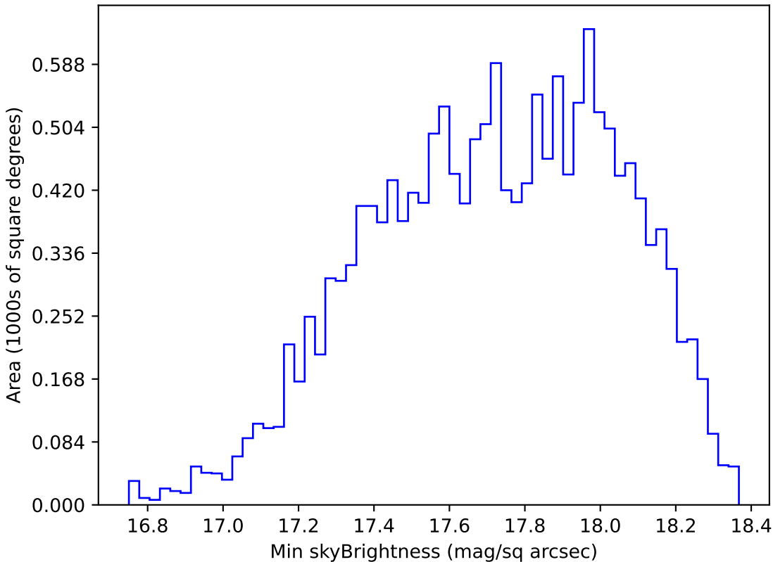
baseline_v3.0_10yrs WFD z band: Min skyBrightness
