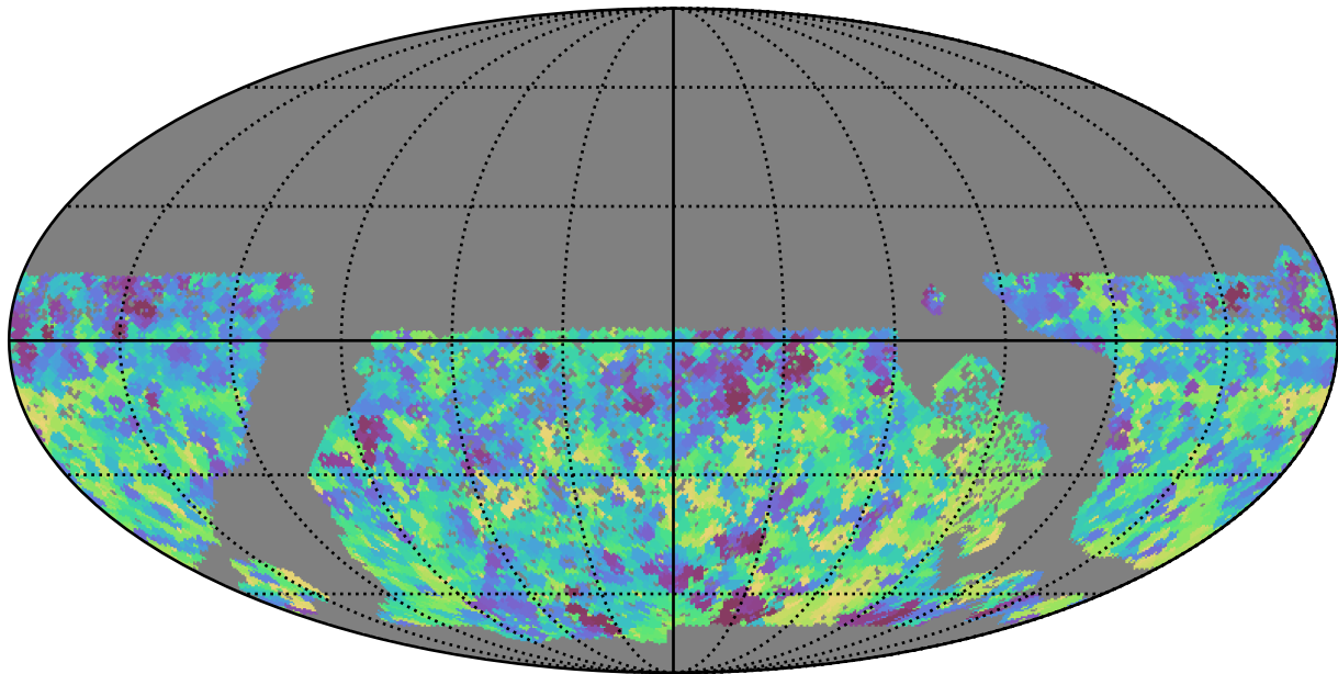
baseline_v3.0_10yrs WFD y band: Min skyBrightness
