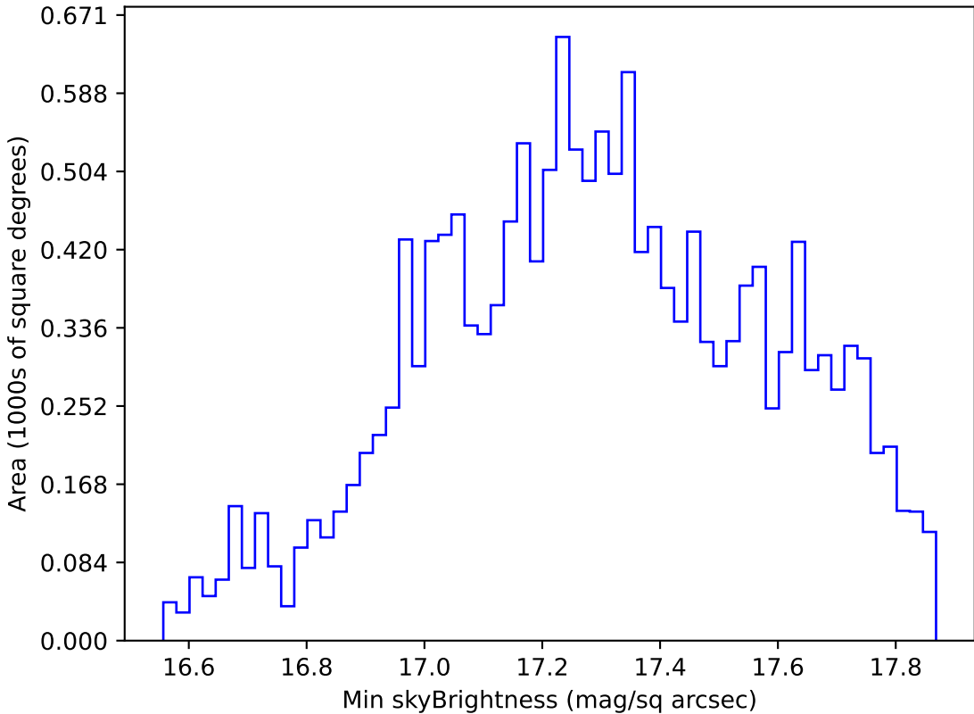
baseline_v3.0_10yrs WFD y band: Min skyBrightness
