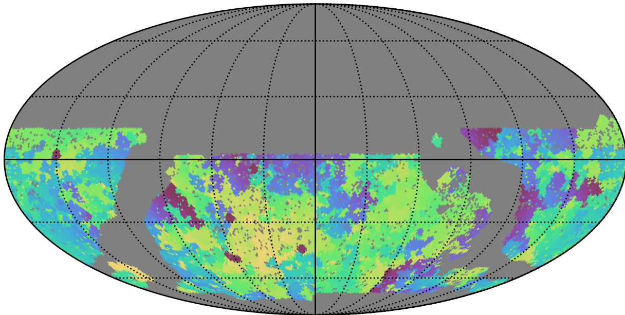
baseline_v3.0_10yrs WFD u band: Min skyBrightness
