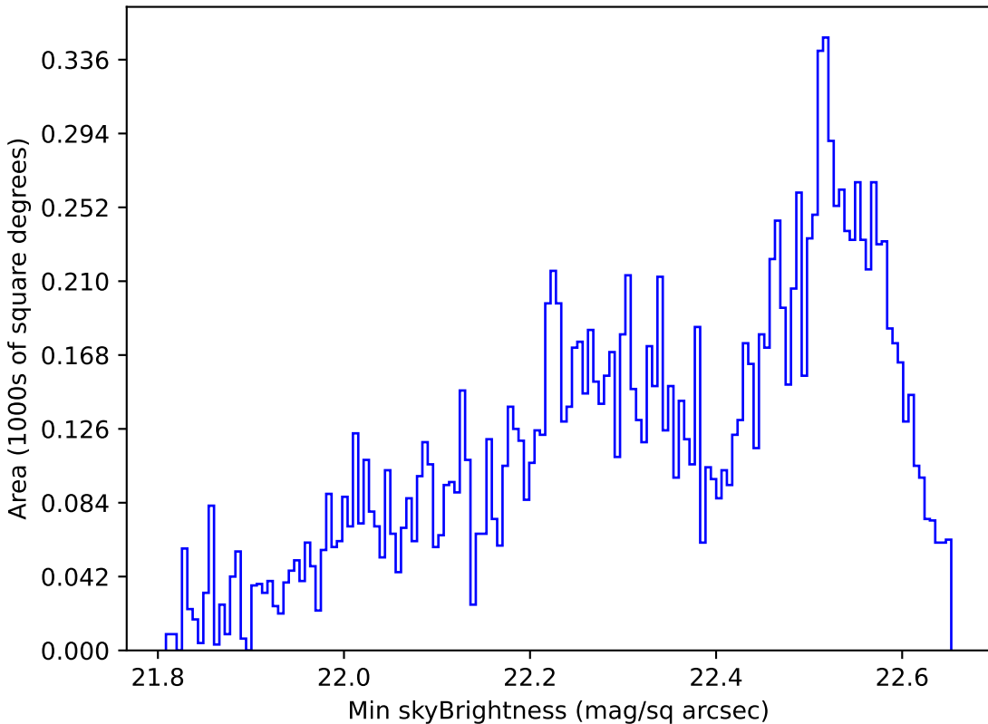
baseline_v3.0_10yrs WFD u band: Min skyBrightness
