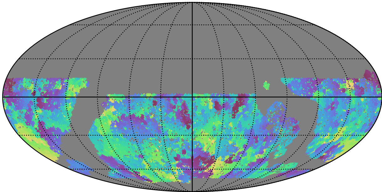
baseline_v3.0_10yrs WFD r band: Min skyBrightness
