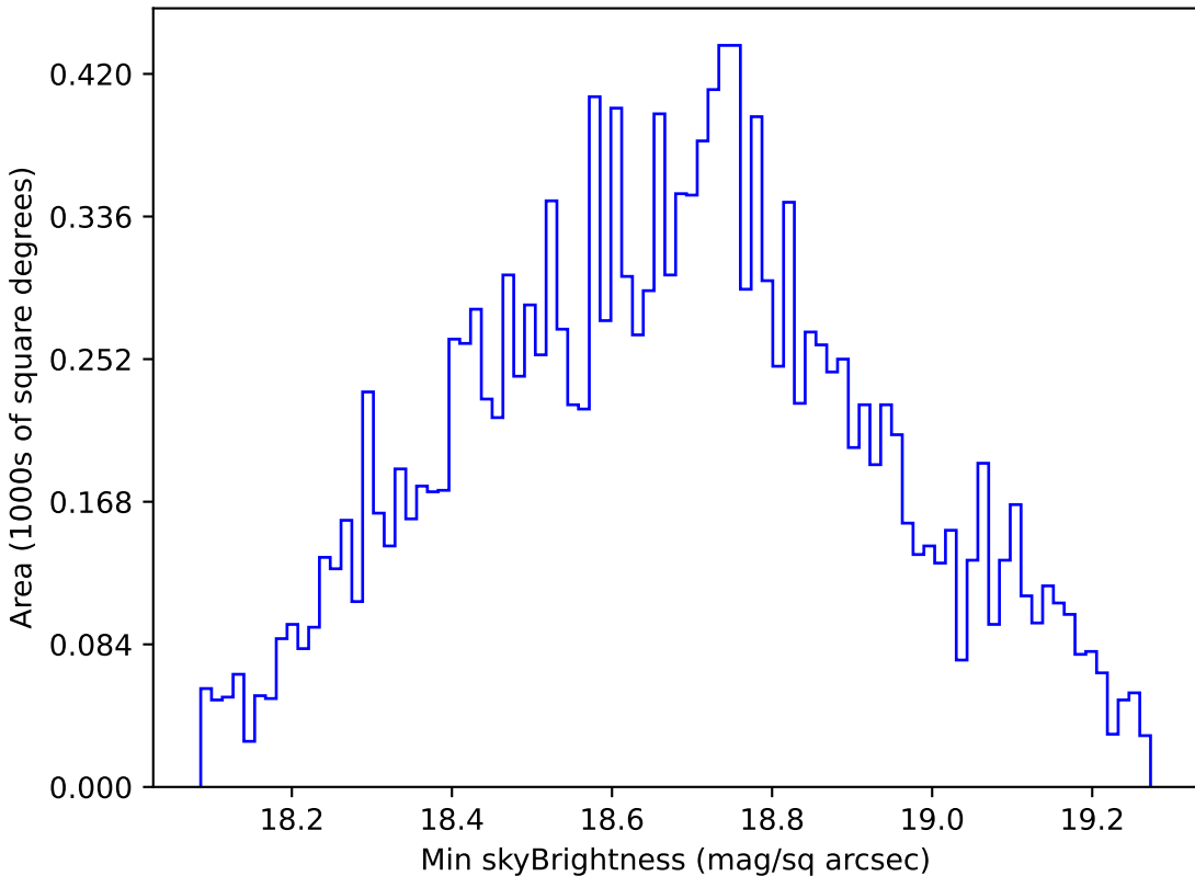
baseline_v3.0_10yrs WFD r band: Min skyBrightness
