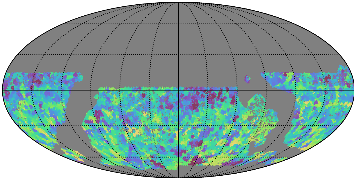
baseline_v3.0_10yrs WFD all bands: Min skyBrightness
