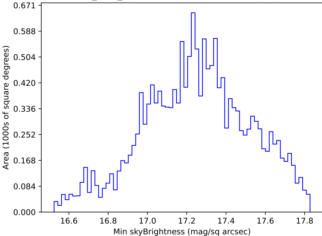
baseline_v3.0_10yrs WFD all bands: Min skyBrightness
